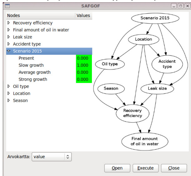
Figure 1. The plug-in dialog box. The “slow growth” option is set to occur at probability 1. “Arvokartta” is for selecting the value layer.
